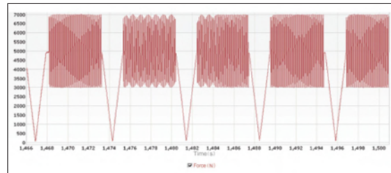
waveforms superimposed on sine and trapezoidal waveforms
